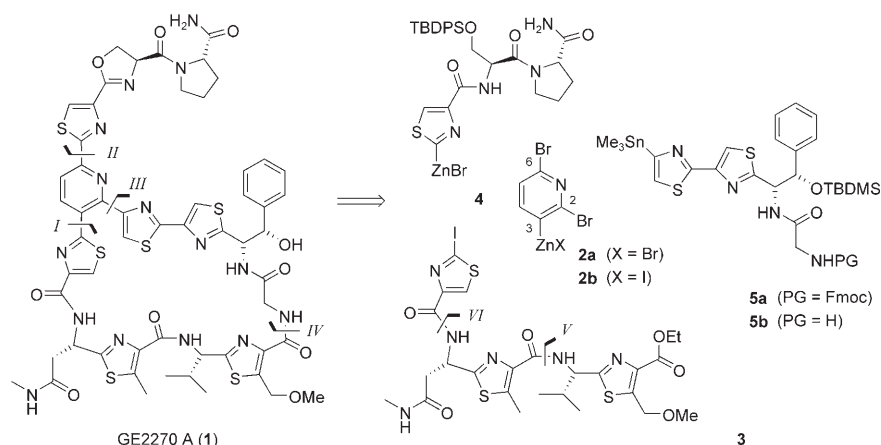
Scheme 1. Synthetic strategy for the construction of the thiazolyl peptide GE2270 A ( 1 ) by regioselective cross-coupling reactions. Fmoc = 9-Fluorenylmethoxycarbonyl, PG = protecting group, TBDMS = tert -butyldimethylsilyl, TBDPS = tert -Butyldiphenylsilyl.
