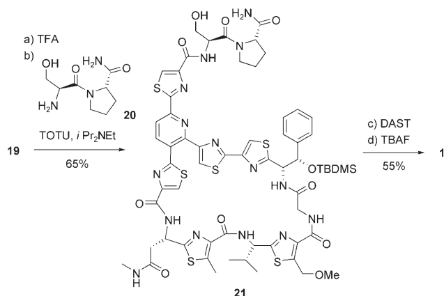
Scheme 5. Completion of the total synthesis of GE2270 A ( 1 ). Reaction conditions: a) TFA/ \text{CH}_2\text{Cl}_2 (1:9), 25 °C, 2 h; b) 20 (4 equiv), TOTU (1.5 equiv), i\text{Pr}_2\text{NEt} (10 equiv), DMF, 25 °C, 4 h, 65% yield over two steps; c) DAST (26 equiv), \text{CH}_2\text{Cl}_2 , −78 °C, 1 h; d) TBAF (2.5 equiv), THF, 25 °C, 2 h, 55% yield over two steps. DAST = (diethylamino)sulfur trifluoride, TBAF = tetrabutylammonium fluoride, TOTU = \text{O}-[(\text{ethoxycarbonyl})\text{cyanomethyl}(\text{amino})-N,N,N',N' -tetramethyluronium tetrafluoroborate.
