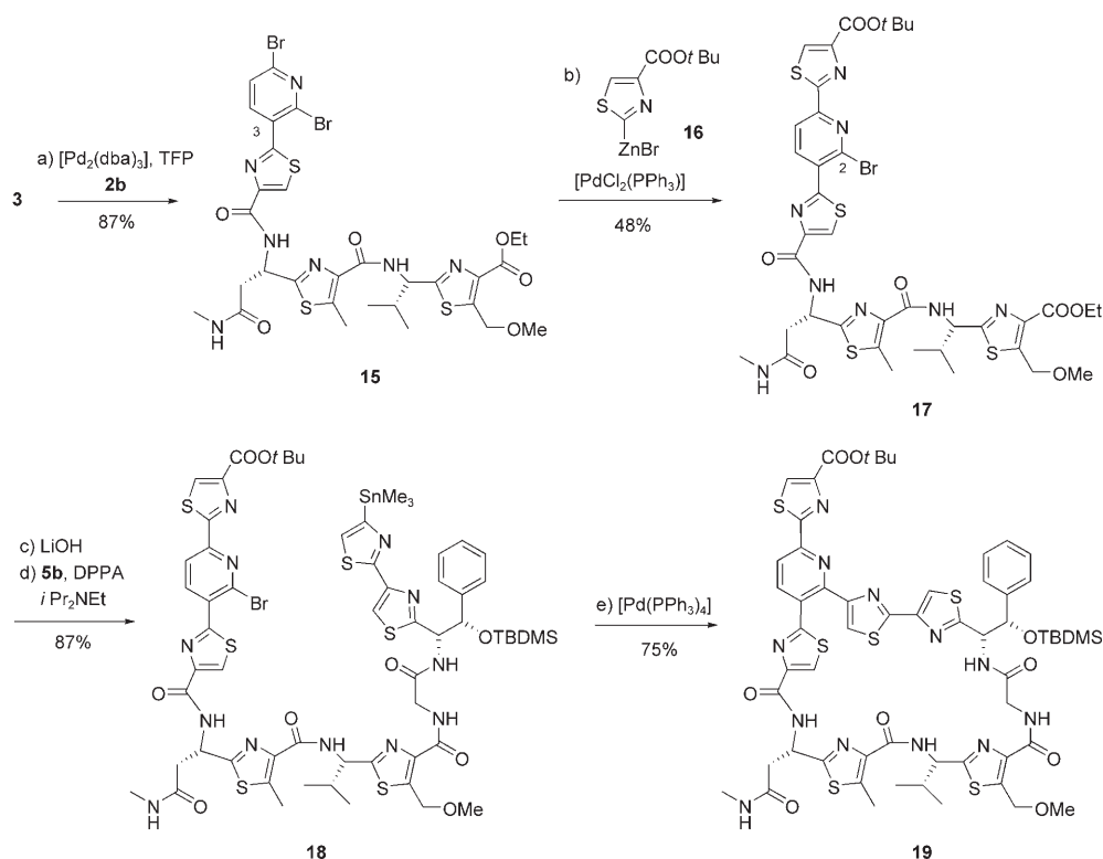
Scheme 4. Regioselective introduction of the pyridine substituents by cross-coupling and formation of macrolactam 19 . Reaction conditions: a) 2b (3 equiv), [\text{Pd}_2(\text{dba})_3] (6 mol %), TFP (12 mol %), THF/DMA (5:1), 45 °C, 16 h, 87%; b) 16 (8 equiv), [\text{PdCl}_2(\text{PPh}_3)_2] (30 mol %), DMA, 45 °C, 3.5 h, 48%; c) 1 M LiOH/ tert -BuOH/THF (1:2:1), 25 °C, 1 h; d) 5b (1 equiv), DPPA (1.7 equiv), i\text{Pr}_2\text{NEt} (3.4 equiv), DMF, 25 °C, 16 h, 87% yield over two steps; e) [\text{Pd}(\text{PPh}_3)_4] (20 mol %), toluene (1 mL \mu\text{mol}^{-1} ), 85 °C, 75%. dba = Dibenzylideneacetone, DPPA = diphenylphosphoryl azide, TFP = tri(2-furyl)phosphane.
