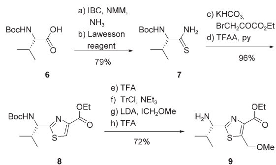
Scheme 2. Synthesis of the valine-derived thiazole 9 . Reaction conditions: a) IBC (1.05 equiv), NMM (1.1 equiv), 25% NH 3 (aq), THF, –20 °C to 25 °C, 16 h, 96%; b) Lawesson reagent (0.5 equiv), THF, 25 °C, 16 h, 82%; c) KHCO 3 (8 equiv), BrCH 2 COCO 2 Et (3 equiv), DME, –15 °C, 24 h; d) TFAA (4.1 equiv), pyridine (8.8 equiv), DME, –15 °C, 2 h, 96% yield over two steps; e) TFA/CH 2 Cl 2 (1:5); f) TrCl (1 equiv), NEt 3 (2.6 equiv), DME, 25 °C, 16 h, 98% yield over two steps; g) LDA (1.1 equiv), THF, –78 °C, 1 min, then ICH 2 OCH 3 (3 equiv), –78 °C, 5 min, 74%; h) TFA/CH 2 Cl 2 (1:5). DME = dimethoxyethane, IBC = isobutyl chloroformate, LDA = lithium diisopropylamide, NMM = N -methylmorpholine, py = pyridine, TFAA = trifluoroacetic anhydride, TFA = trifluoroacetic acid, TrCl = trityl chloride.
